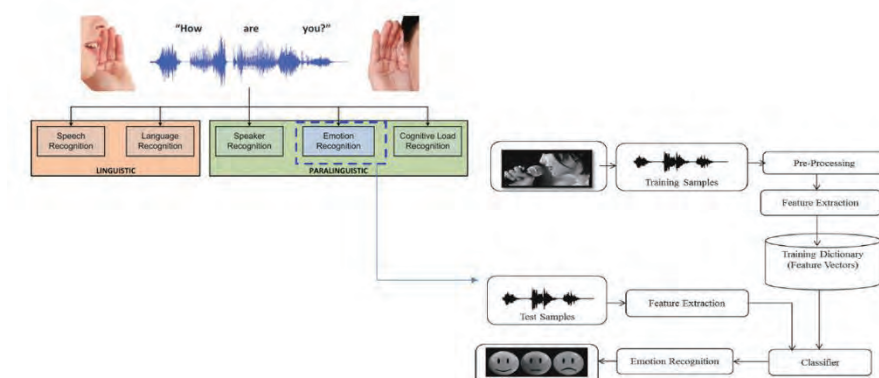
Figure 3. Speech pattern-based emotion classification scheme.
