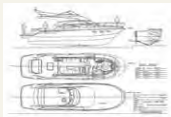
CAD (computer-aided design) of 15m boat
