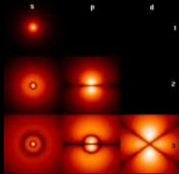
Electron/ Positron
