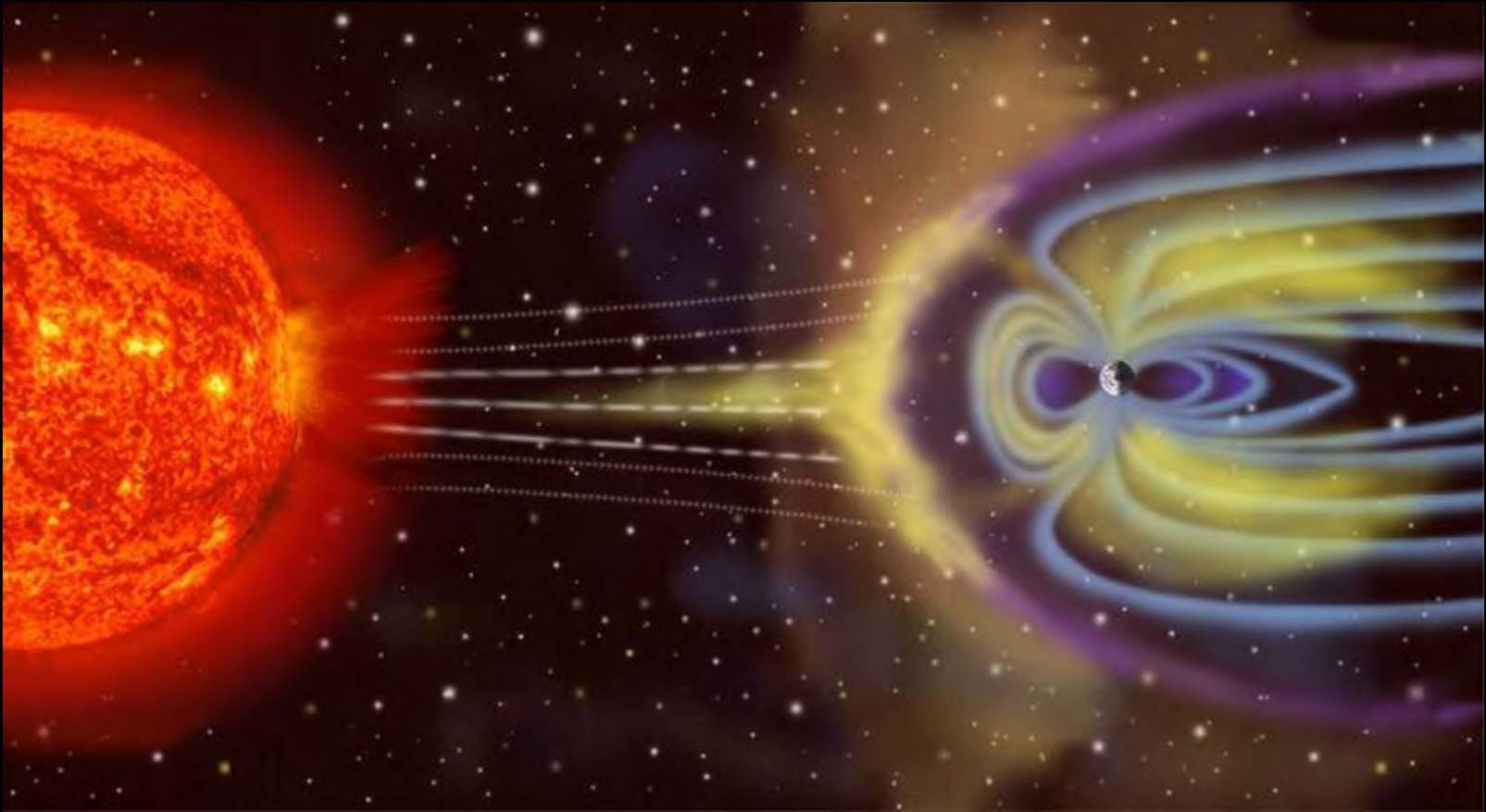
Beauty of Sun and Earths Magnetic field
