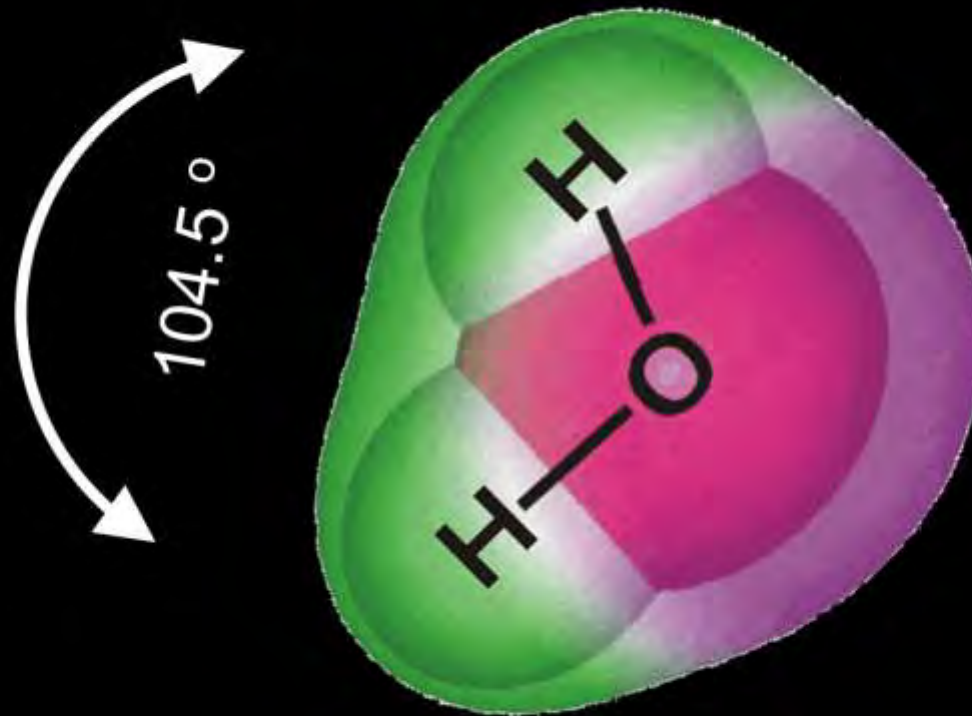
Water molecule
